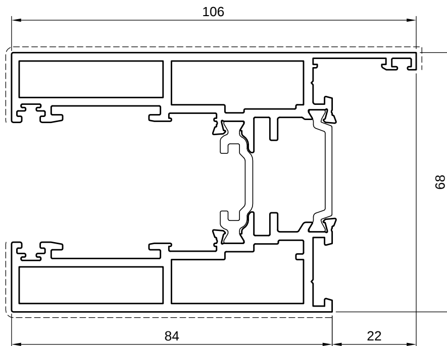
5TT11016 kg/ml 3,286 sup. in vista 230mm
