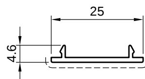
5ST11063 kg/ml 0,106 sup. in vista 28mm
