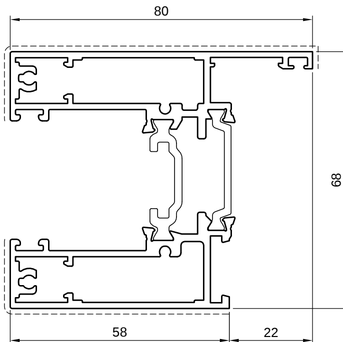
5TT11029 Elegance kg/ml 2,195 sup. in vista 179mm
