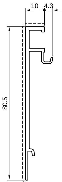
5ST11020 kg/ml 0,536 sup. in vista 90,5mm
