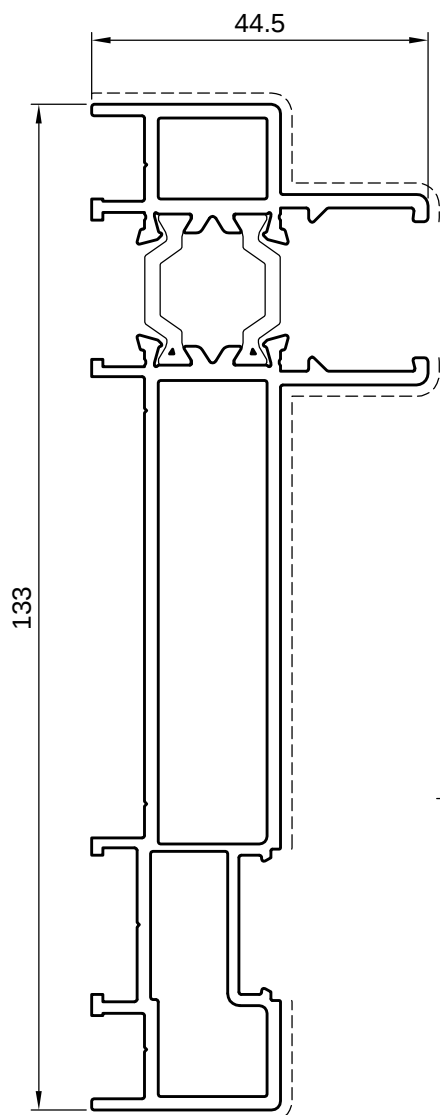
5TT11014 kg/ml 2,131 sup. in vista 180mm
