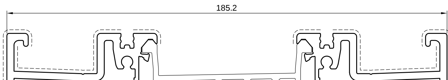
* 5TT11028 kg/ml 2,521 sup. in vista 256mm
