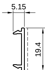
5AB70003 kg/ml 0,092 sup. in vista 19mm
