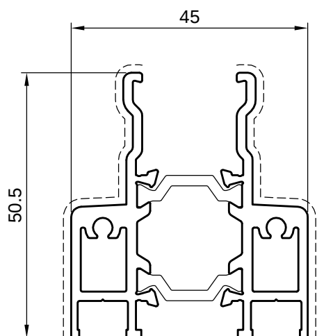
5TT11010 kg/ml 1,326 sup. in vista 128mm
