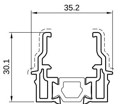
5TT11005 kg/ml 0,706 sup. in vista 50mm
