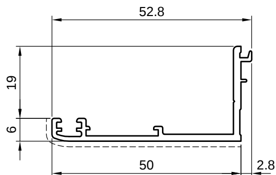
5AT45169 kg/ml 0,392 sup. in vista 55mm
