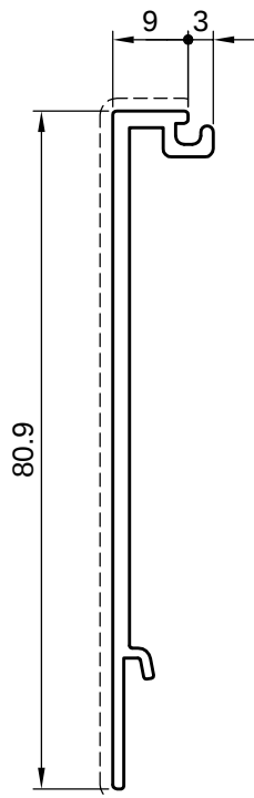
5ST11065 kg/ml 0,498 sup. in vista 91mm
