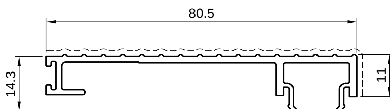
5ST11059 kg/ml 0,589 sup. in vista 97mm
