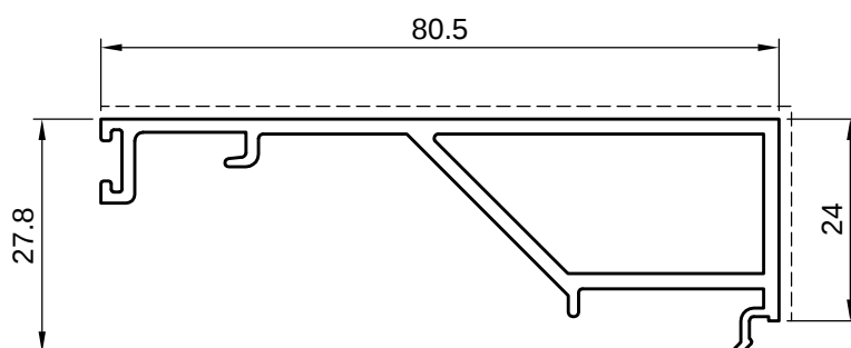
5ST11058 kg/ml 0,826 sup. in vista 140.5mm
