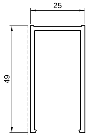
5ST11064 kg/ml 0,645 sup. in vista 102mm
