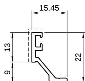
5ST11057 kg/ml 0,170 sup. in vista 17.5mm
