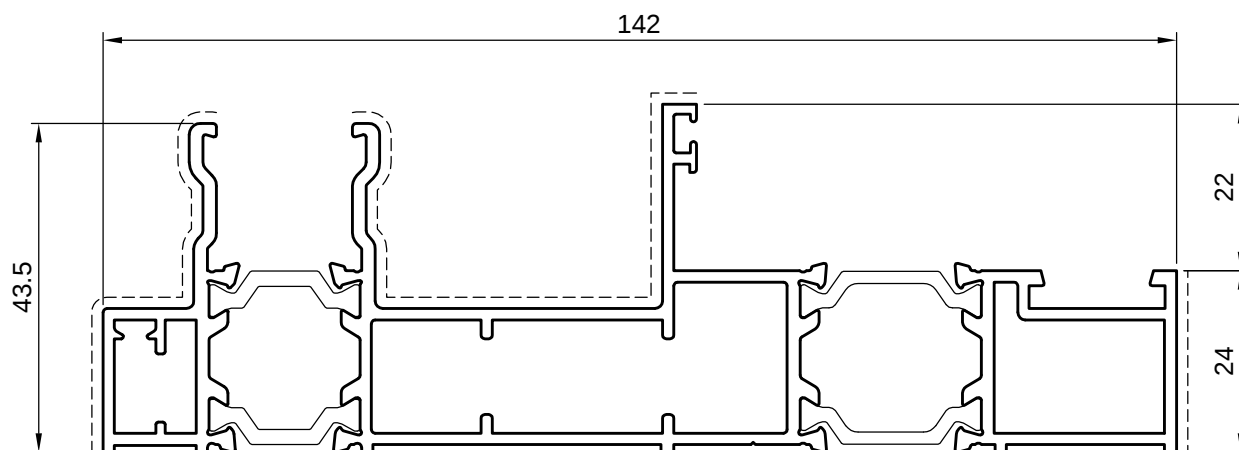
5TT11024 kg/ml 2,355 sup. in vista 176mm
