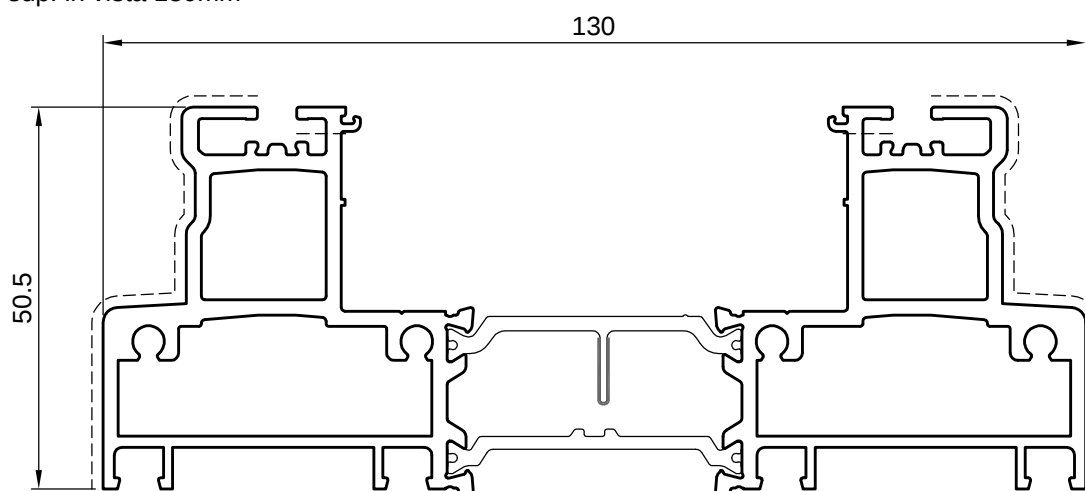
5TT11015 5TT11015 EVO kg/ml 2,885 sup. in vista 154mm
