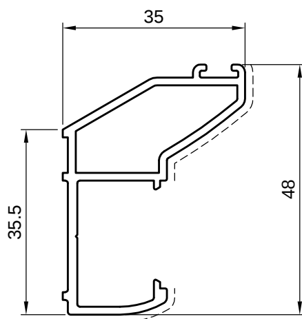
5ST11018 kg/ml 0,609 sup. in vista 53mm
