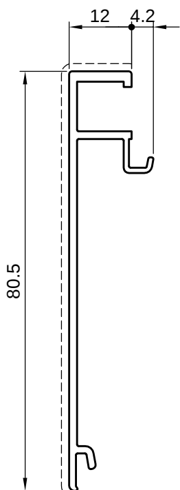
5ST11068 Elegance kg/ml 0,480 sup. in vista 91,5mm
