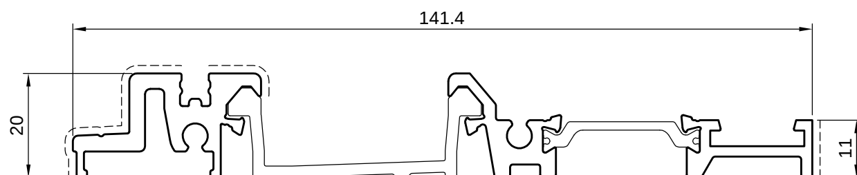
5TT11025 kg/ml 1,649 sup. in vista 71mm
