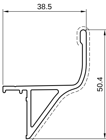
5ST11021 kg/ml 0,583 sup. in vista 70mm
